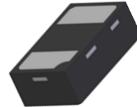
DFN1006-2L (Bottom View)
