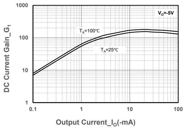
DC Current Gain vs. Output Current
